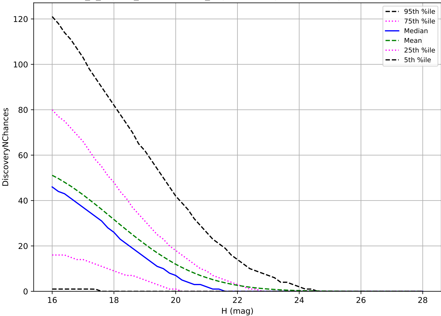
internal_u_expt45_nscale1.1v3.4_10yrs: PHA 3 pairs in 15 nights detection loss
