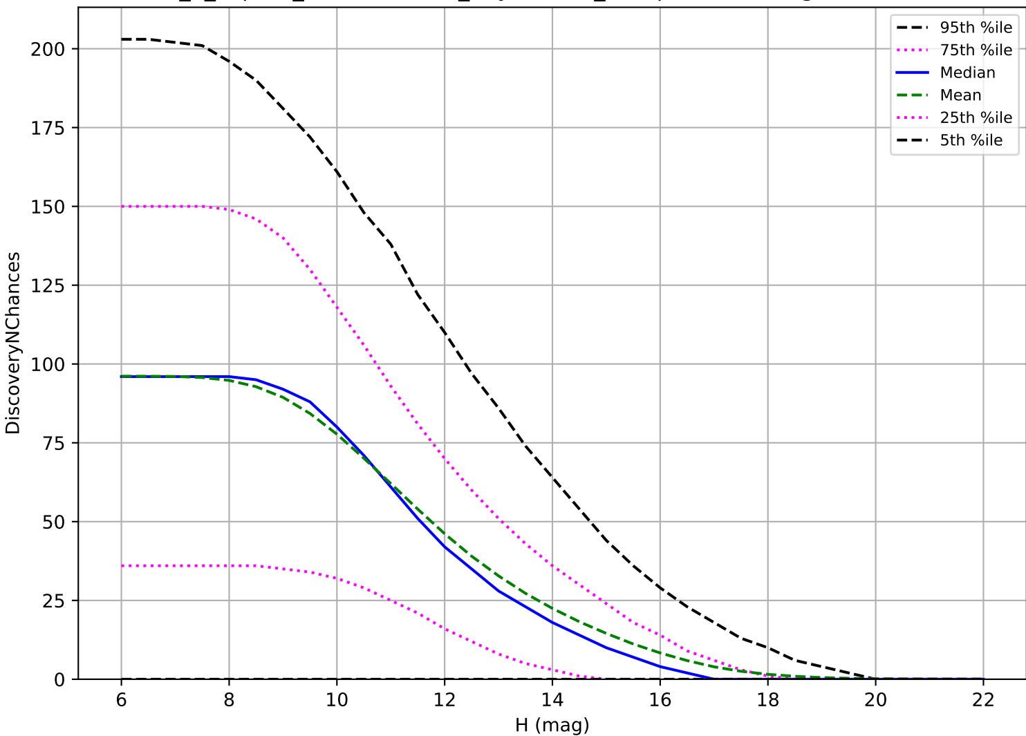
internal_u_expt45_nscale1.1v3.4_10yrs: OCC_r5 3 pairs in 15 nights detection loss
