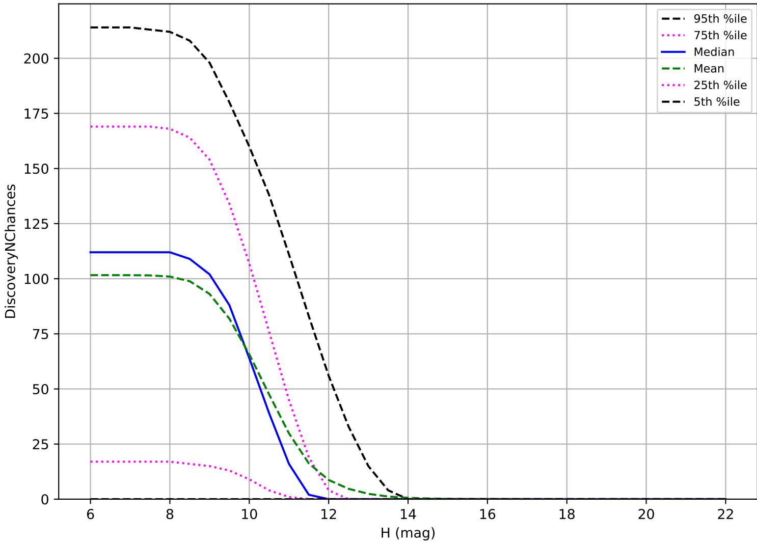
internal_u_expt45_nscale1.1v3.4_10yrs: OCC_r20 3 pairs in 15 nights detection loss
