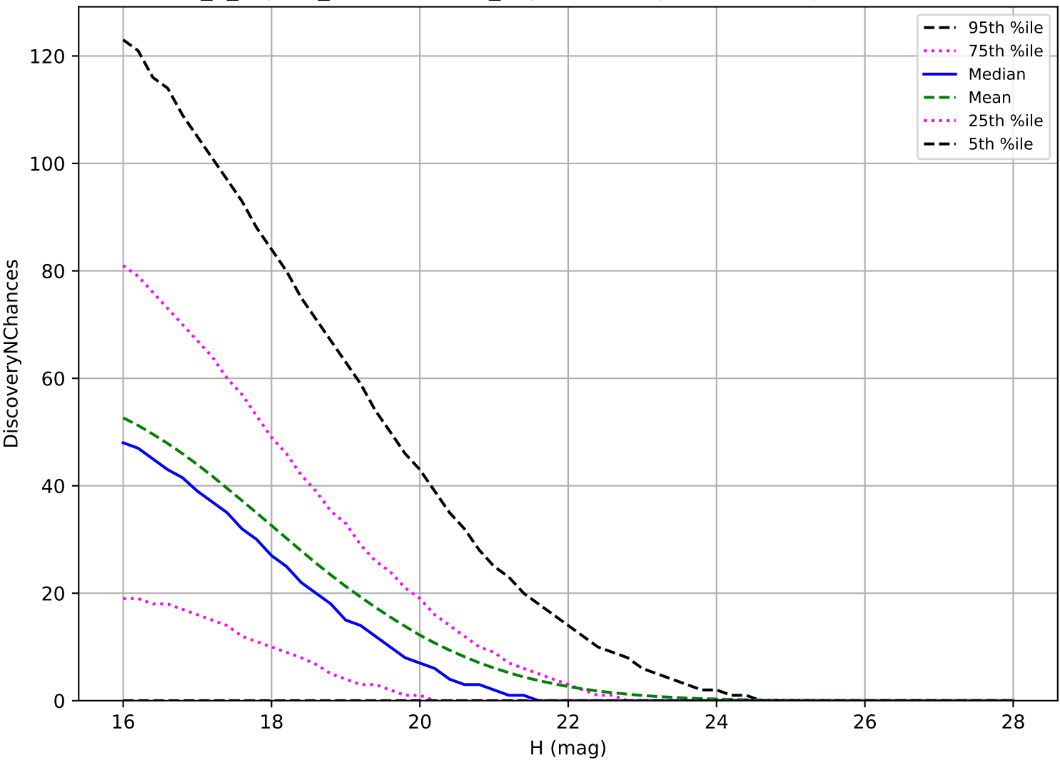
internal_u_expt45_nscale1.1v3.4_10yrs: NEO 3 pairs in 15 nights detection loss
