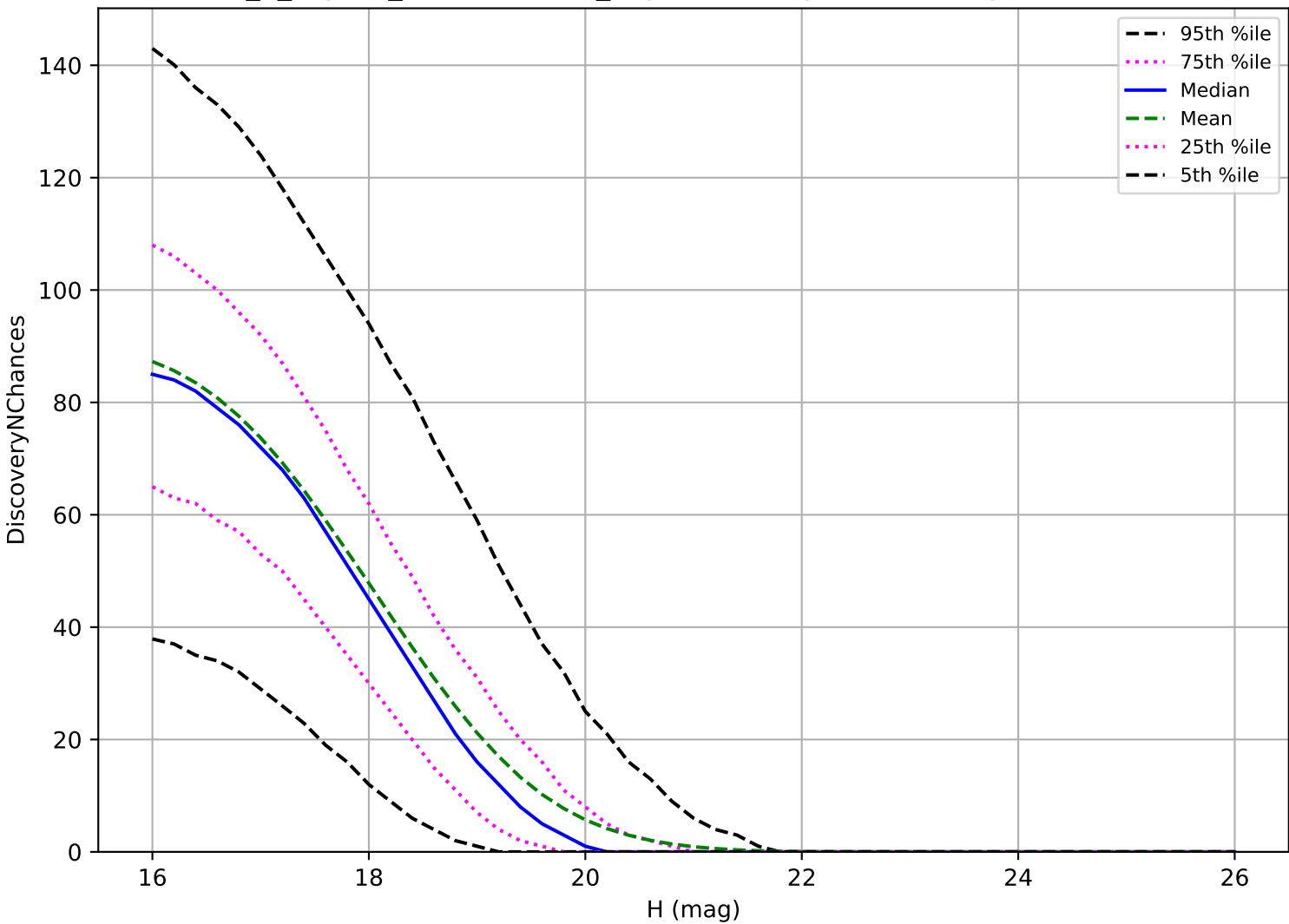
internal_u_expt45_nscale1.1v3.4_10yrs: MBA 3 pairs in 15 nights detection loss
