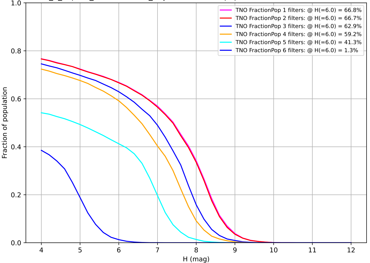
internal_u_expt45_nscale1.1v3.4_10yrs: Fraction of population with colors in X filters TNO
