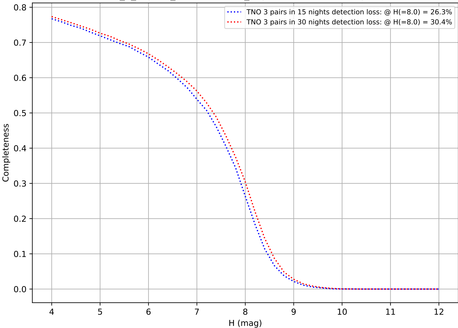
internal_u_expt45_nscale1.1v3.4_10yrs: DifferentialCompleteness
