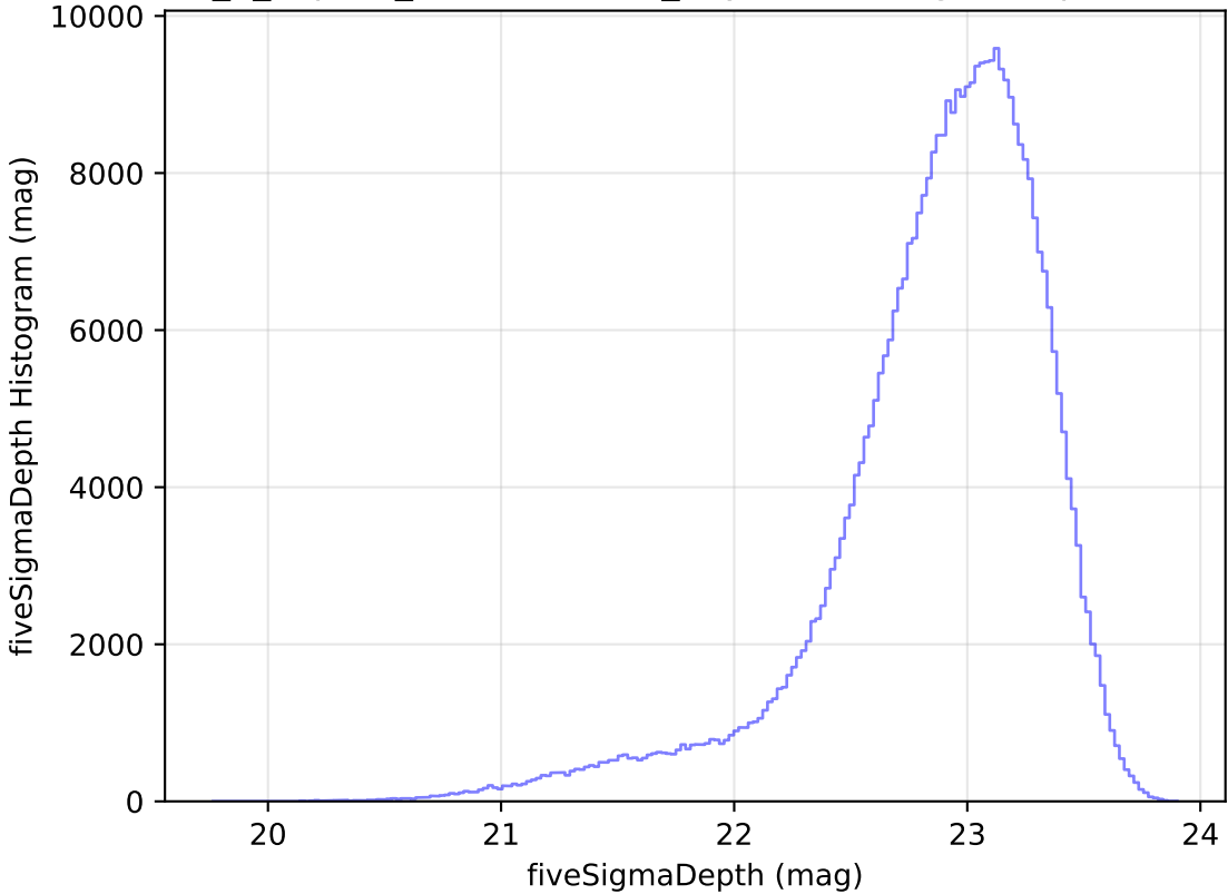
internal_u_expt45_nscale1.1v3.4_10yrs z: fiveSigmaDepth Histogram
