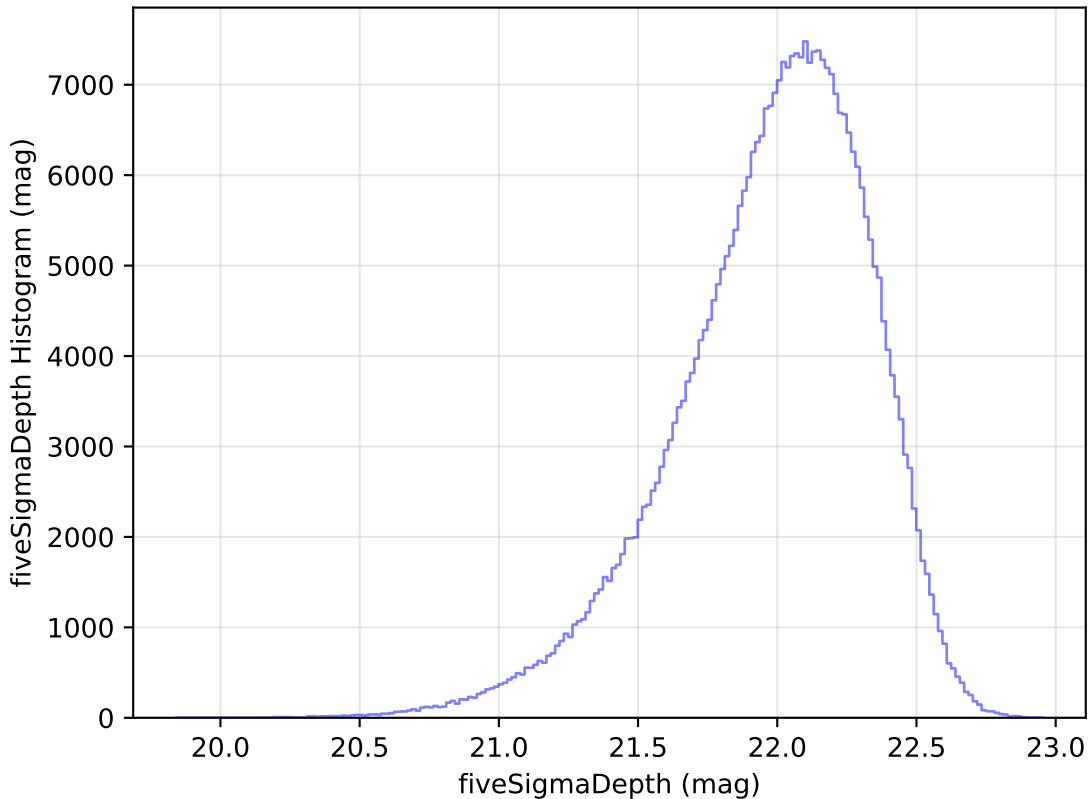
internal_u_expt45_nscale1.1v3.4_10yrs y: fiveSigmaDepth Histogram
