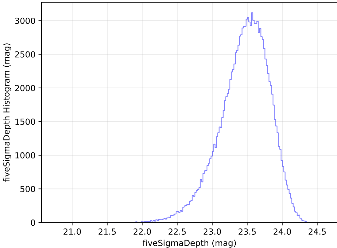
internal_u_expt45_nscale1.1v3.4_10yrs u: fiveSigmaDepth Histogram
