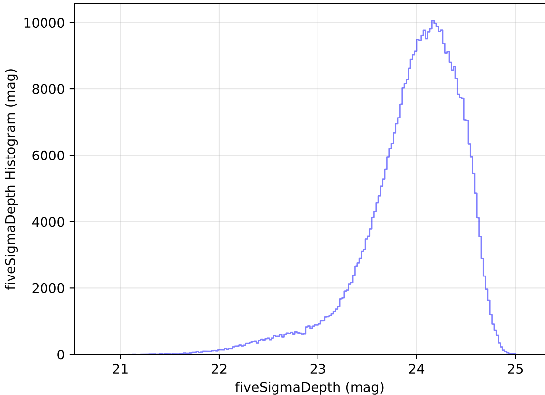
internal_u_expt45_nscale1.1v3.4_10yrs r: fiveSigmaDepth Histogram
