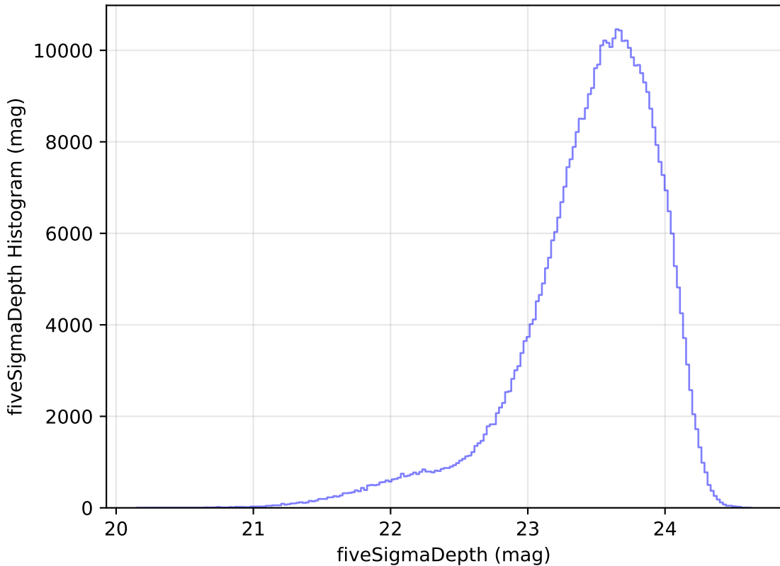
internal_u_expt45_nscale1.1v3.4_10yrs i: fiveSigmaDepth Histogram
