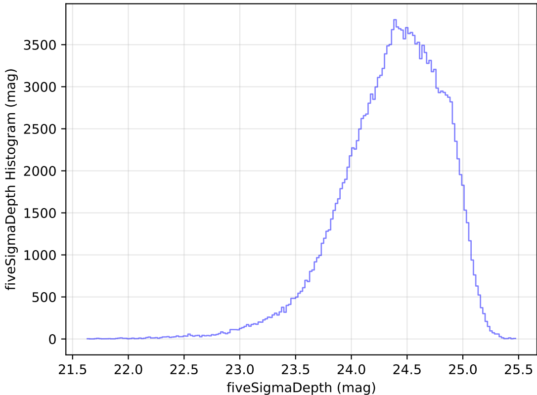
internal_u_expt45_nscale1.1v3.4_10yrs g: fiveSigmaDepth Histogram
