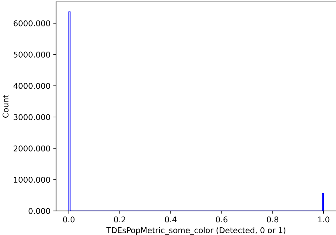
internal_u_expt45_nscale1.1v3.4_10yrs : TDEsPopMetric_some_color
