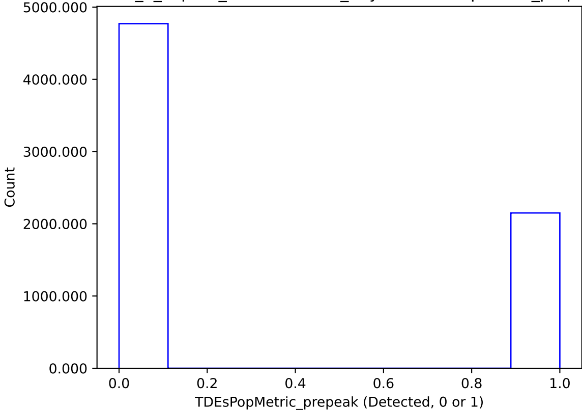
internal_u_expt45_nscale1.1v3.4_10yrs : TDEsPopMetric_prepeak
