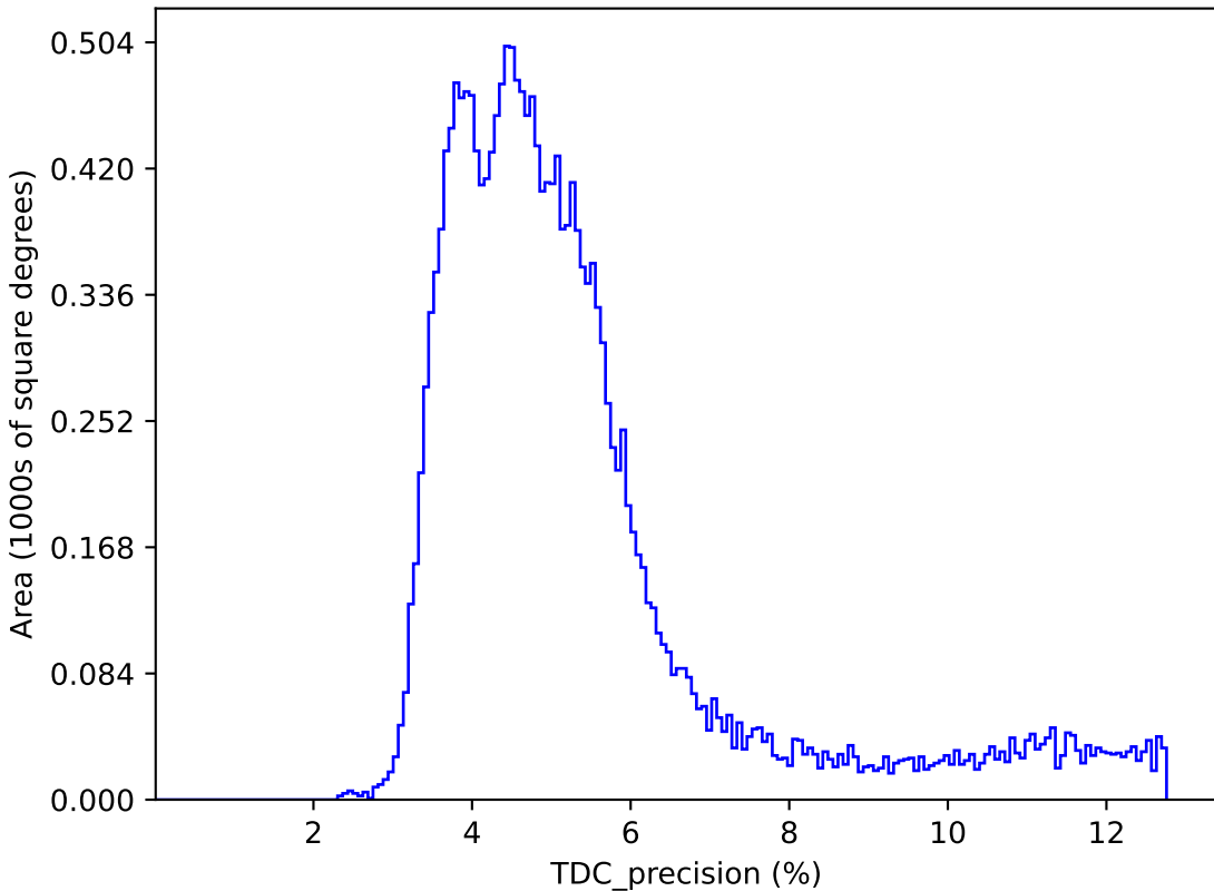
internal_u_expt45_nscale1.1v3.4_10yrs : TDC_precision
