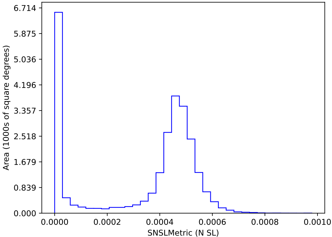
internal_u_expt45_nscale1.1v3.4_10yrs : SNSLMetric
