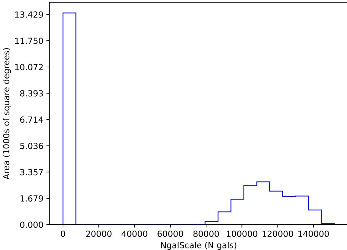
internal_u_expt45_nscale1.1v3.4_10yrs i: NgalScale
