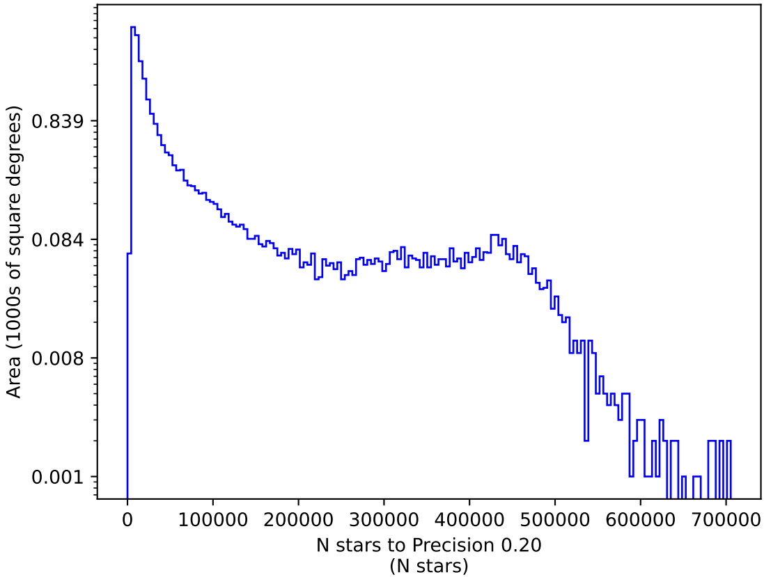
internal_u_expt45_nscale1.1v3.4_10yrs r: N stars to Precision 0.20
