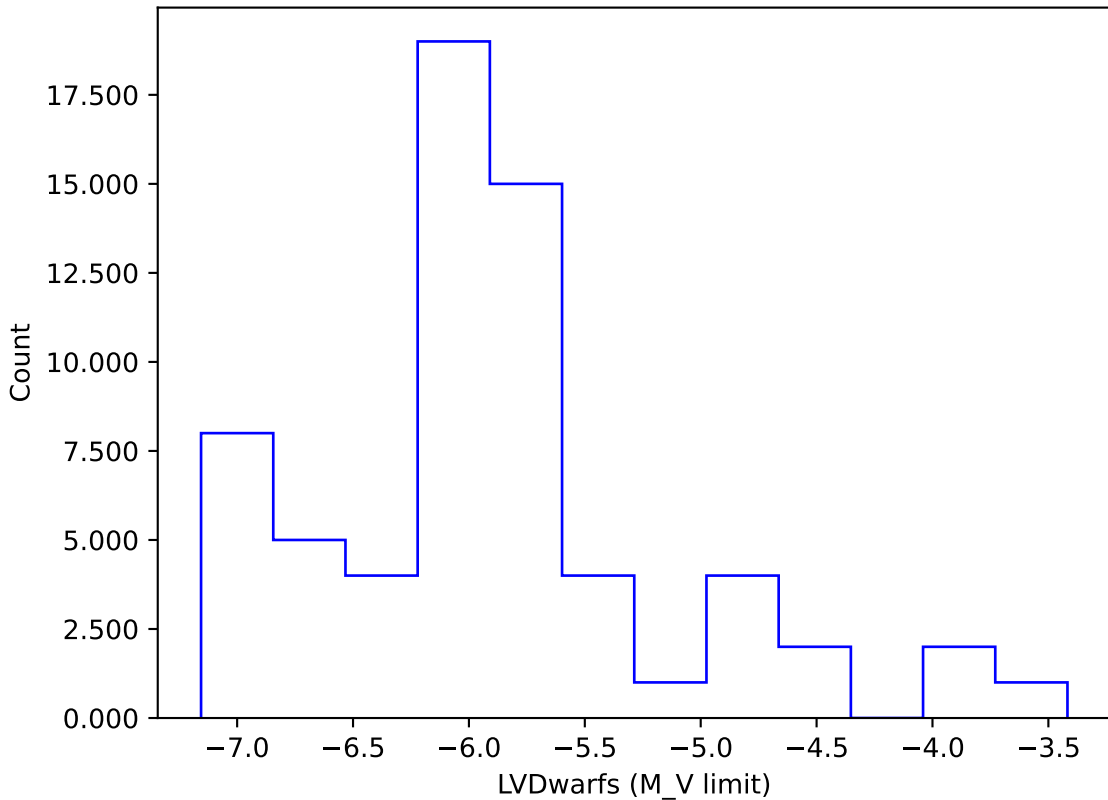
internal_u_expt45_nscale1.1v3.4_10yrs gi: LVDwarfs
