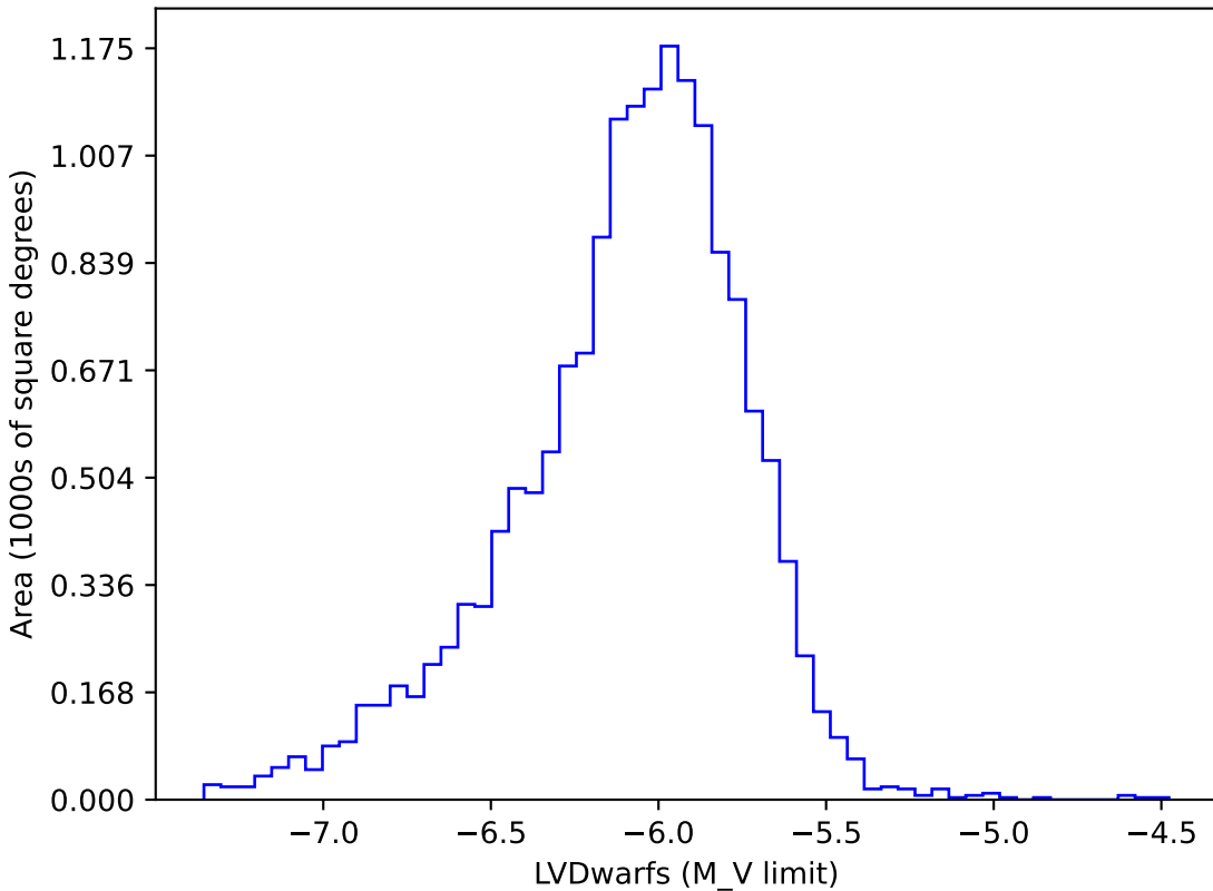
internal_u_expt45_nscale1.1v3.4_10yrs gi: LVDwarfs
