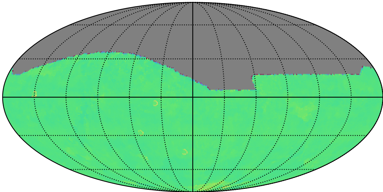
internal_u_expt45_nscale1.1v3.4_10yrs r: Kuiper rotTelPos
