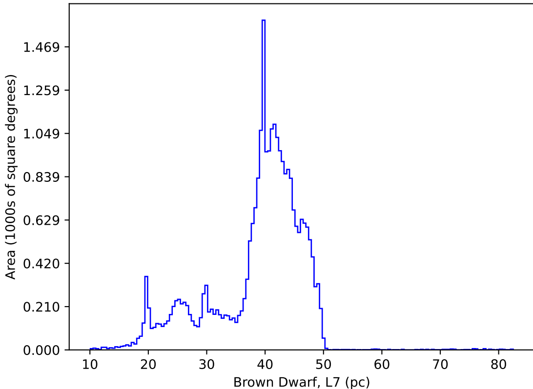
internal_u_expt45_nscale1.1v3.4_10yrs : Brown Dwarf, L7
