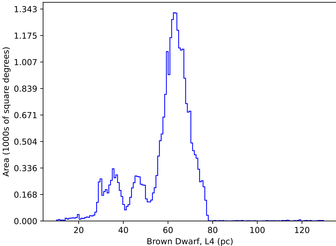
internal_u_expt45_nscale1.1v3.4_10yrs : Brown Dwarf, L4
