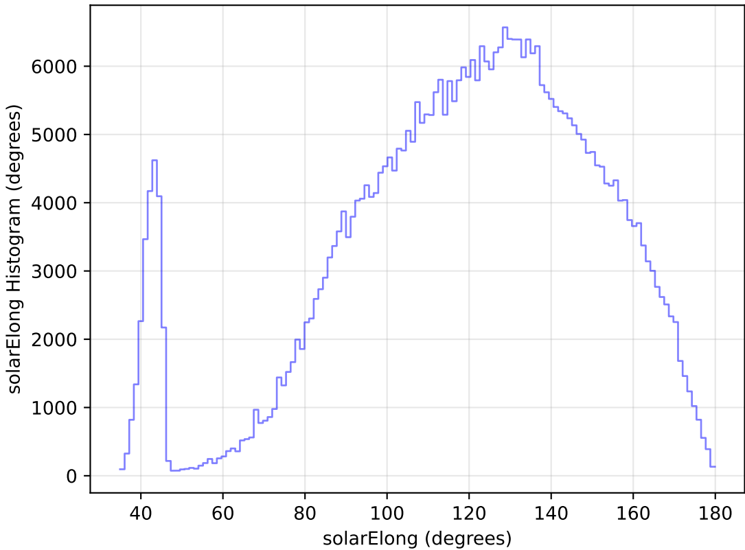
internal_u_expt45_nscale1.1v3.4_10yrs WFD z band: solarElong Histogram
