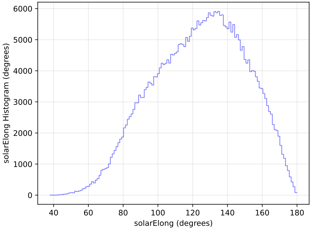
internal_u_expt45_nscale1.1v3.4_10yrs WFD y band: solarElong Histogram
