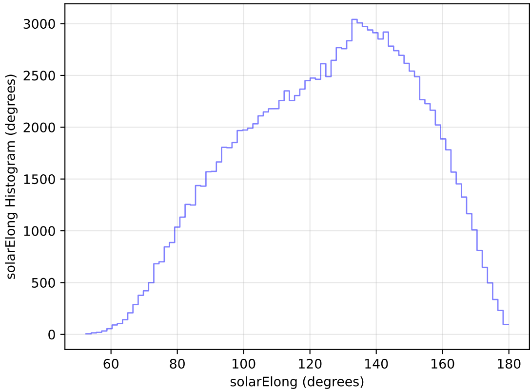
internal_u_expt45_nscale1.1v3.4_10yrs WFD u band: solarElong Histogram
