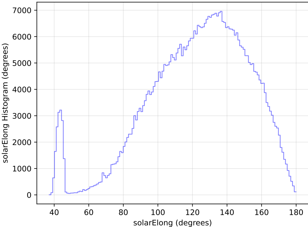
internal_u_expt45_nscale1.1v3.4_10yrs WFD r band: solarElong Histogram
