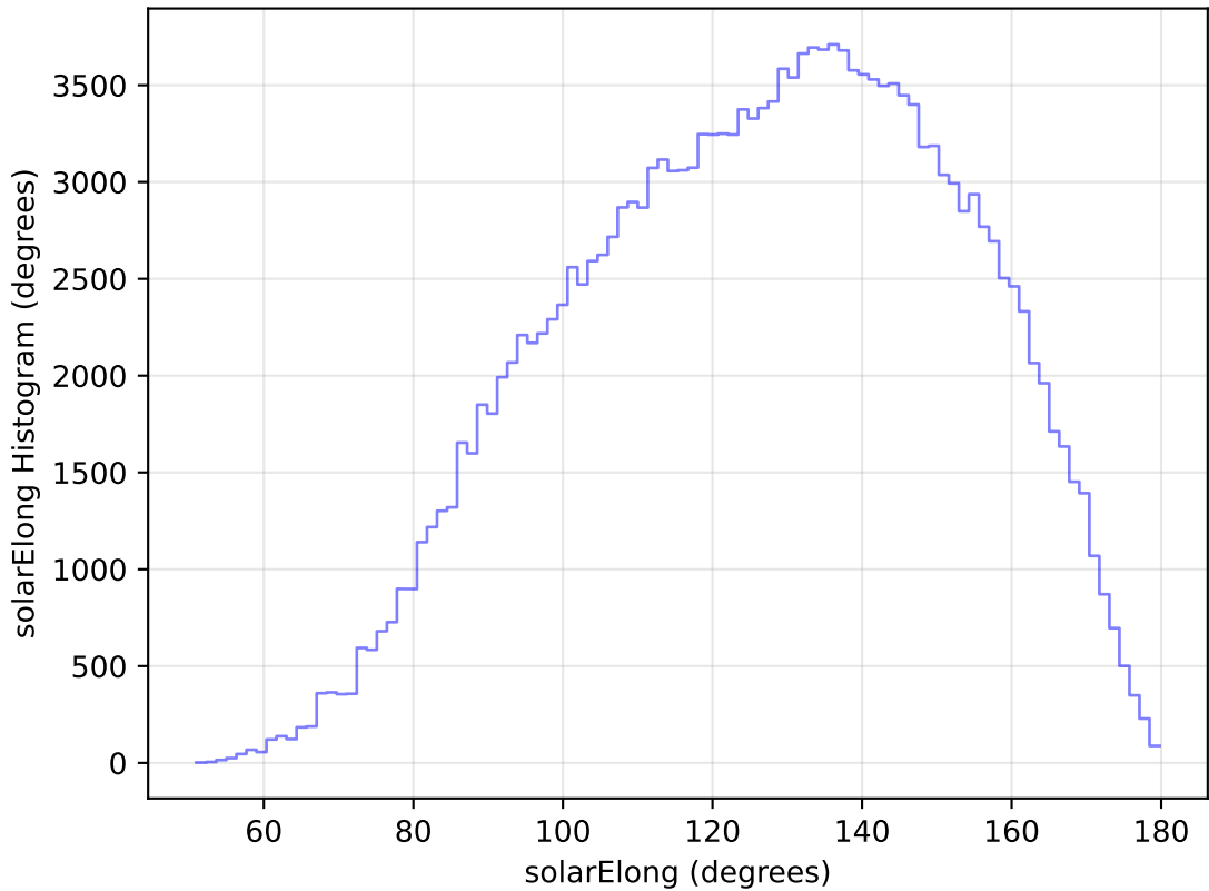
internal_u_expt45_nscale1.1v3.4_10yrs WFD g band: solarElong Histogram
