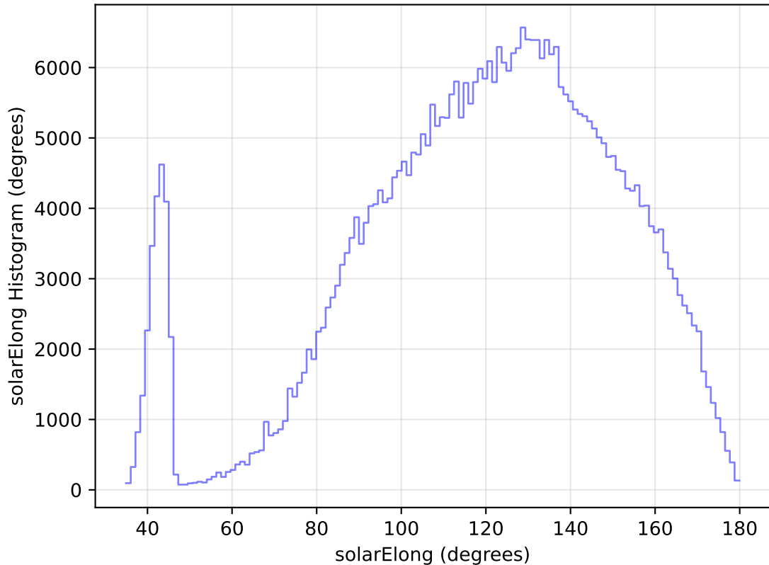
internal_u_expt45_nscale1.1v3.4_10yrs All sky z band: solarElong Histogram
