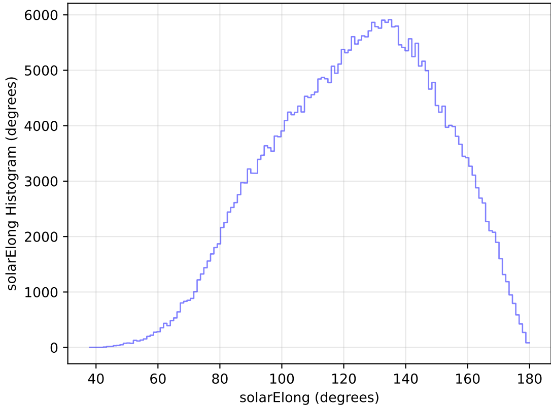
internal_u_expt45_nscale1.1v3.4_10yrs All sky y band: solarElong Histogram
