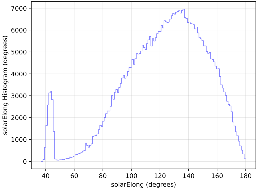
internal_u_expt45_nscale1.1v3.4_10yrs All sky r band: solarElong Histogram
