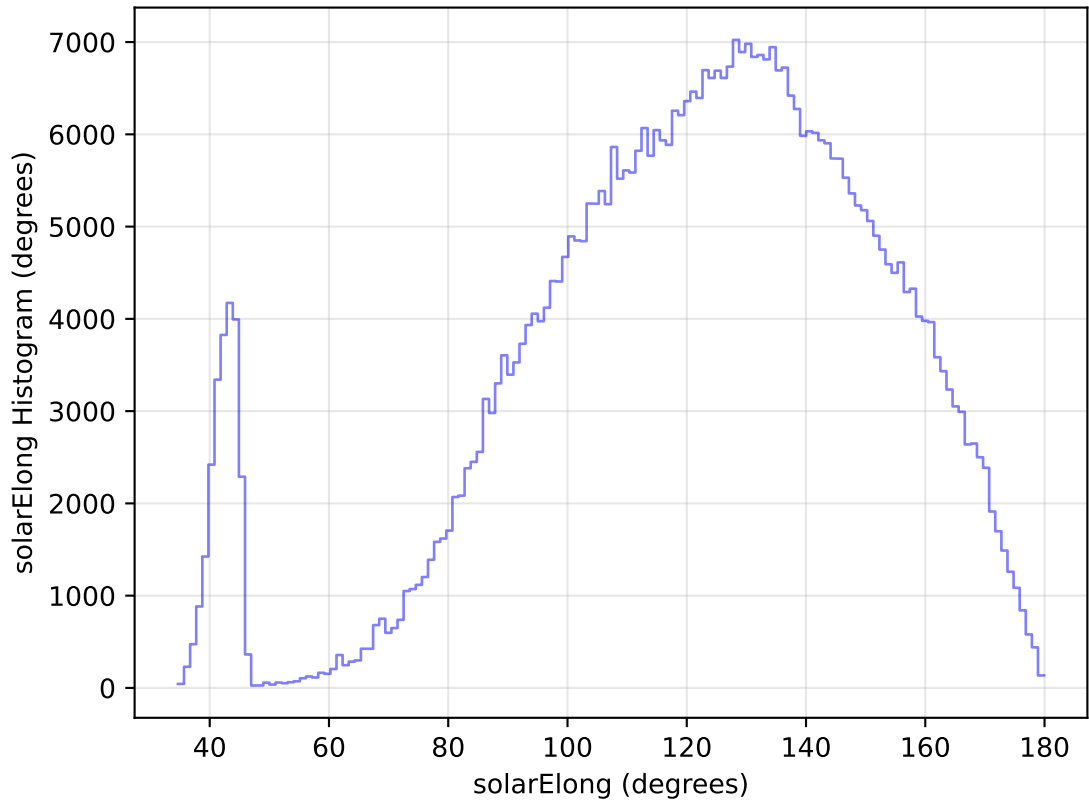
internal_u_expt45_nscale1.1v3.4_10yrs All sky i band: solarElong Histogram
