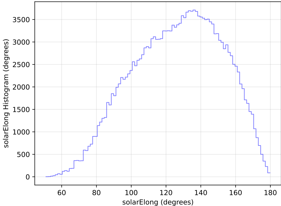
internal_u_expt45_nscale1.1v3.4_10yrs All sky g band: solarElong Histogram
