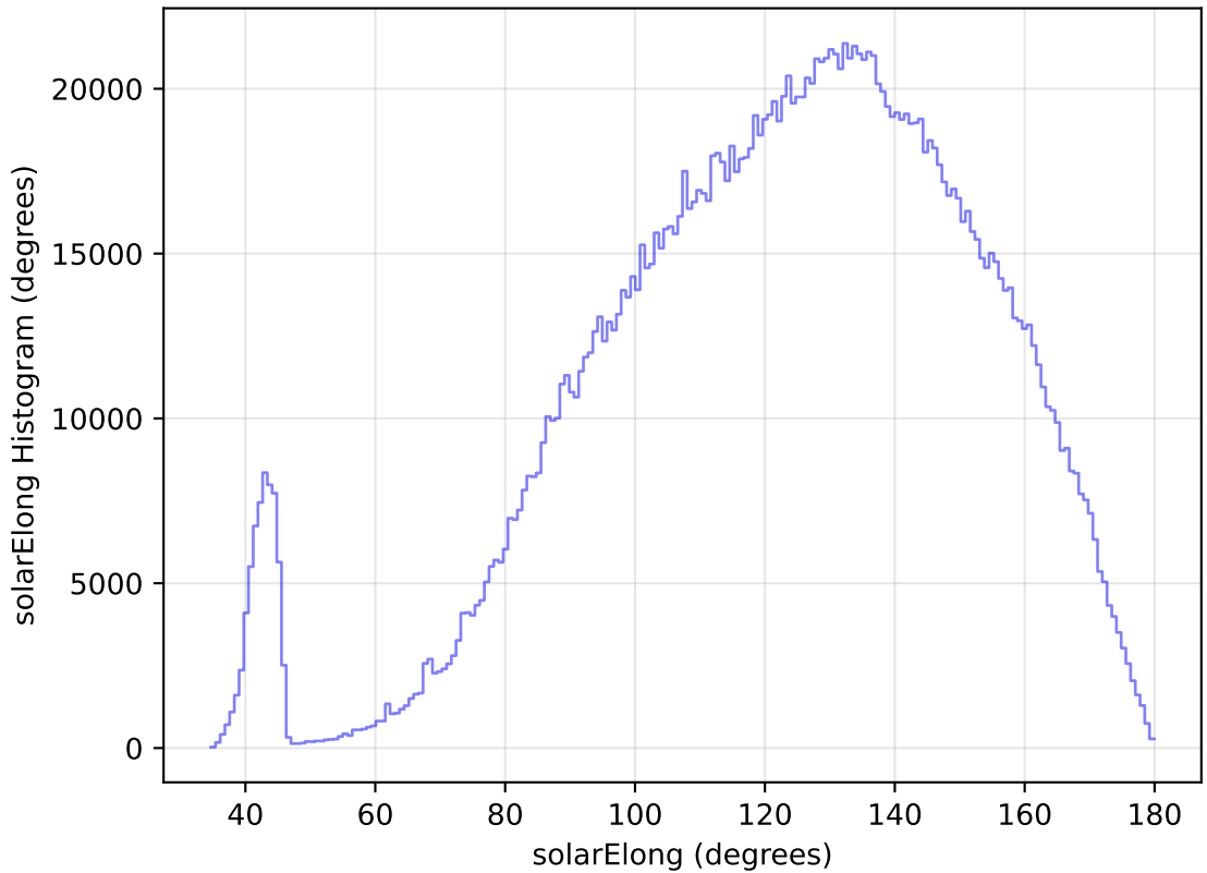
internal_u_expt45_nscale1.1v3.4_10yrs All sky all bands: solarElong Histogram
