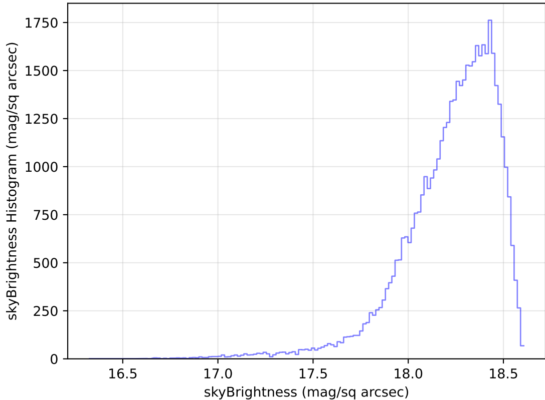
internal_u_expt45_nscale1.1v3.4_10yrs Yr 1 y band: skyBrightness Histogram
