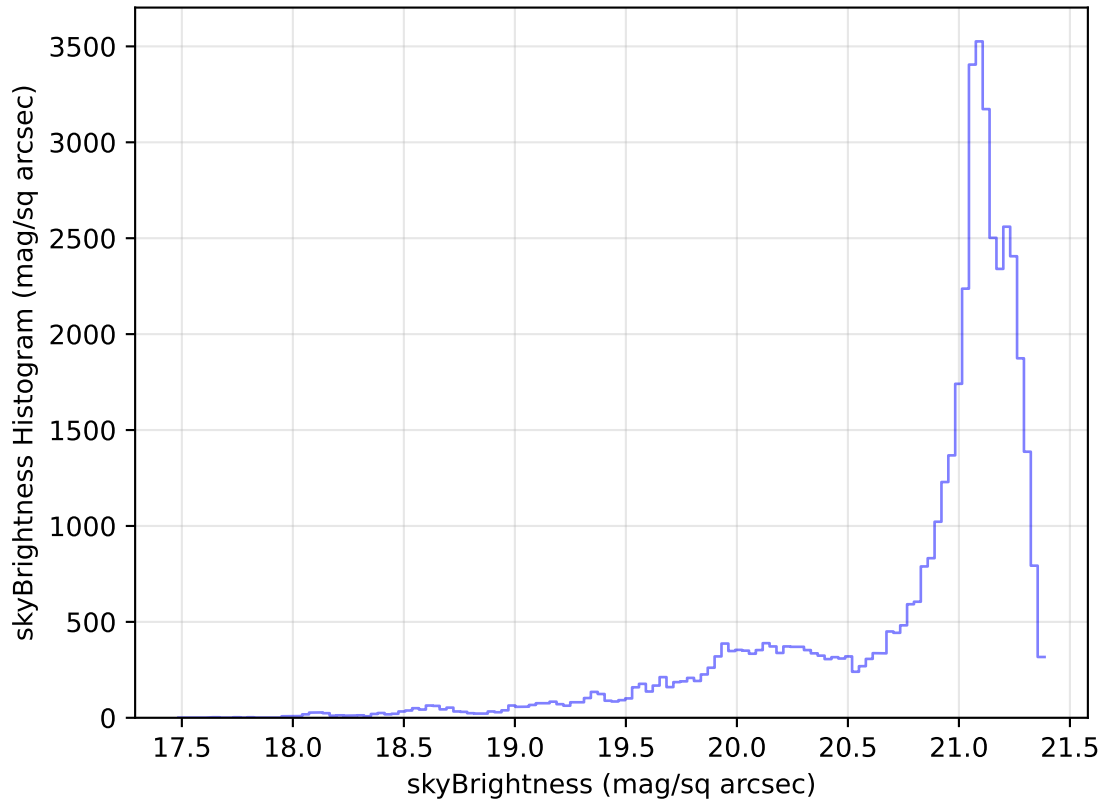
internal_u_expt45_nscale1.1v3.4_10yrs Yr 1 r band: skyBrightness Histogram
