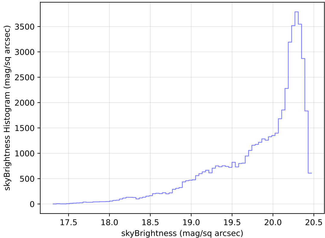
internal_u_expt45_nscale1.1v3.4_10yrs Yr 1 i band: skyBrightness Histogram
