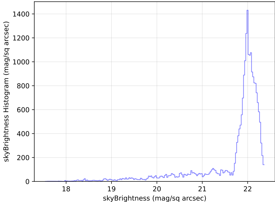
internal_u_expt45_nscale1.1v3.4_10yrs Yr 1 g band: skyBrightness Histogram
