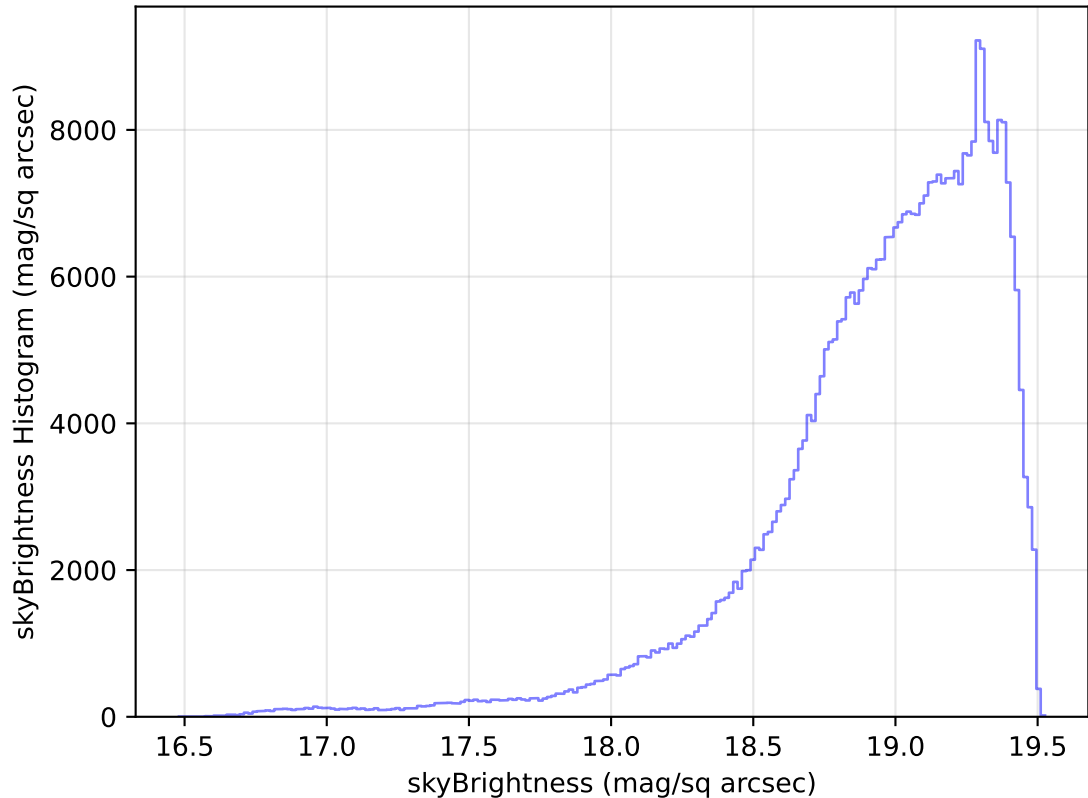
internal_u_expt45_nscale1.1v3.4_10yrs WFD z band: skyBrightness Histogram
