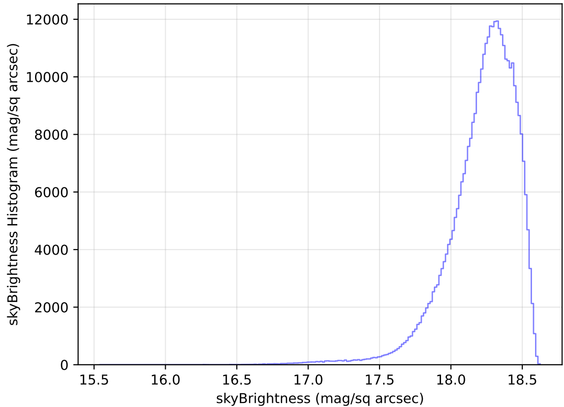
internal_u_expt45_nscale1.1v3.4_10yrs WFD y band: skyBrightness Histogram
