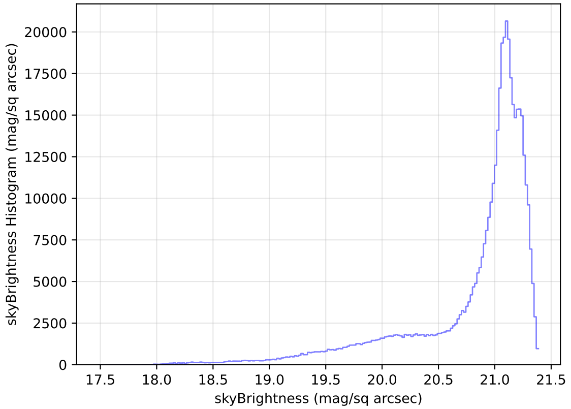
internal_u_expt45_nscale1.1v3.4_10yrs WFD r band: skyBrightness Histogram
