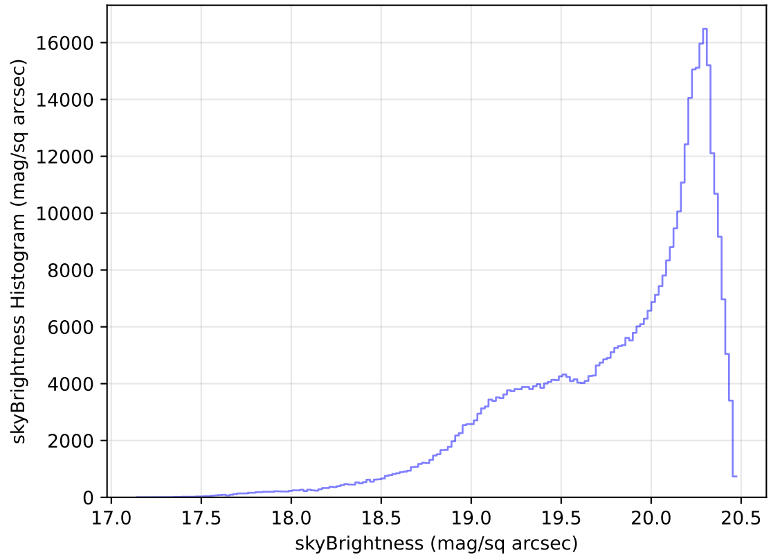
internal_u_expt45_nscale1.1v3.4_10yrs WFD i band: skyBrightness Histogram
