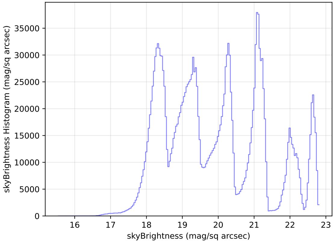
internal_u_expt45_nscale1.1v3.4_10yrs WFD all bands: skyBrightness Histogram
