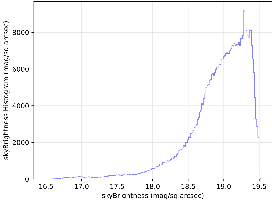
internal_u_expt45_nscale1.1v3.4_10yrs All sky z band: skyBrightness Histogram
