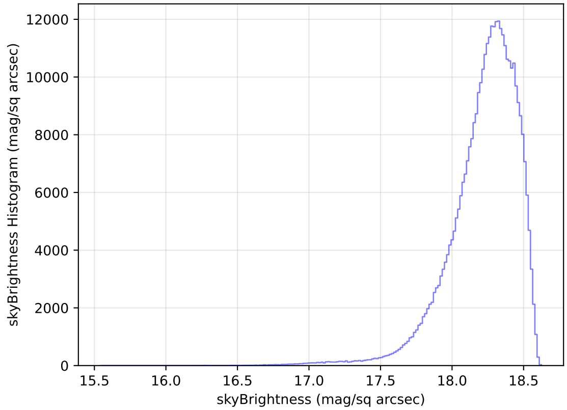
internal_u_expt45_nscale1.1v3.4_10yrs All sky y band: skyBrightness Histogram
