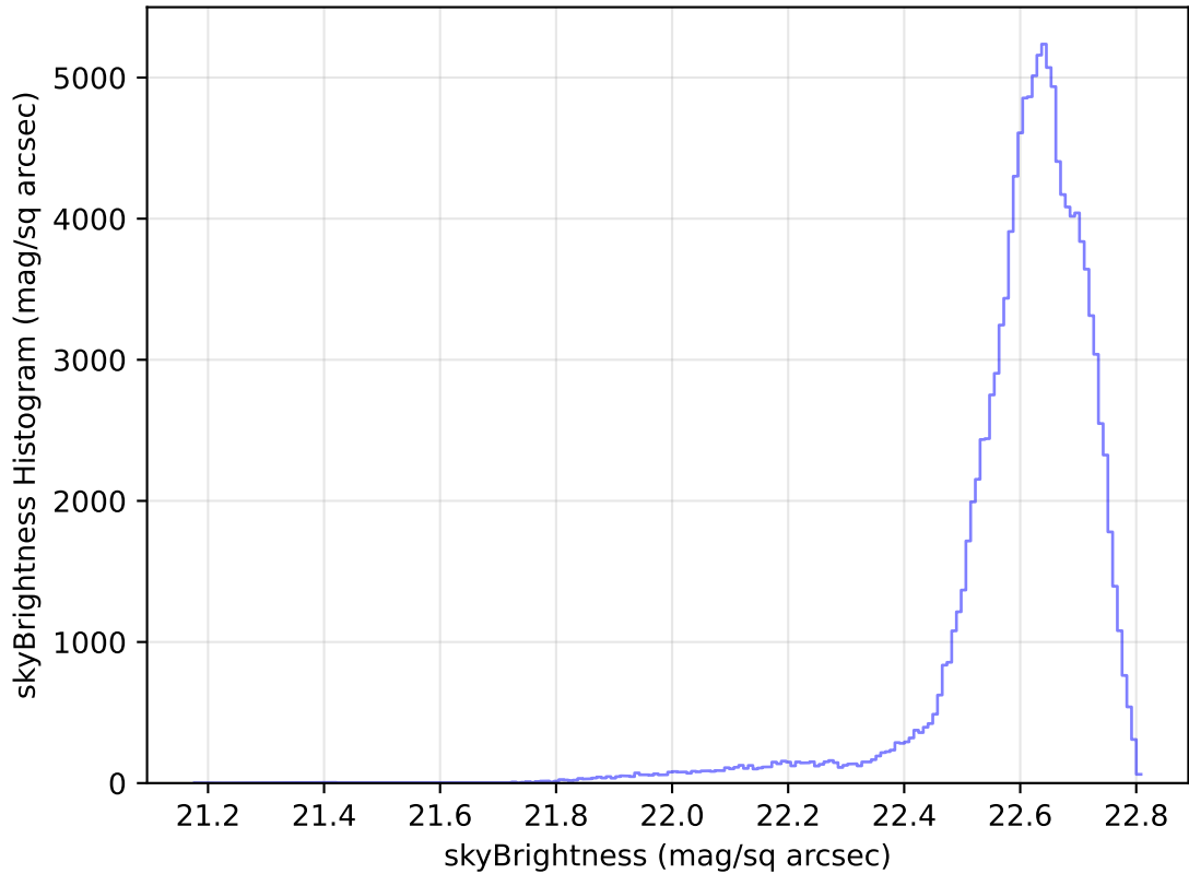
internal_u_expt45_nscale1.1v3.4_10yrs All sky u band: skyBrightness Histogram
