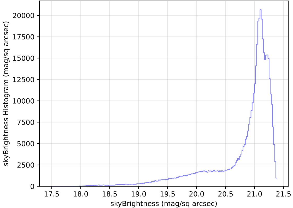
internal_u_expt45_nscale1.1v3.4_10yrs All sky r band: skyBrightness Histogram
