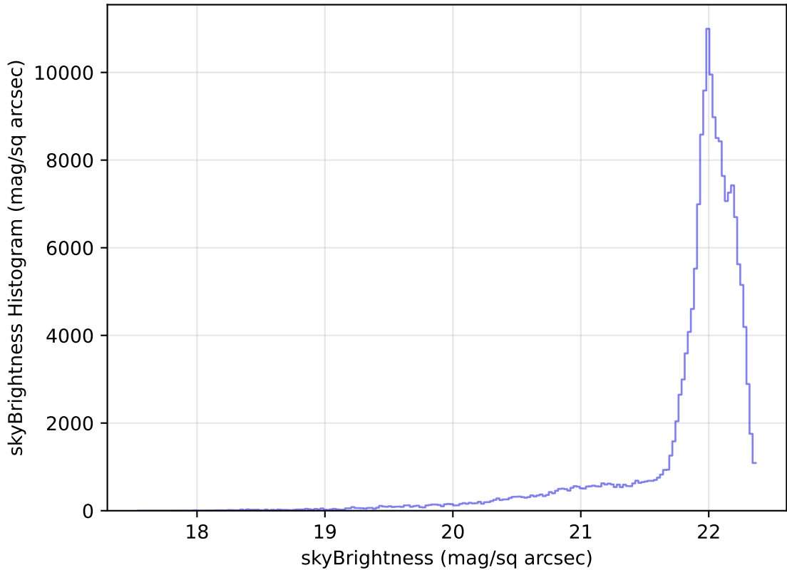
internal_u_expt45_nscale1.1v3.4_10yrs All sky g band: skyBrightness Histogram
