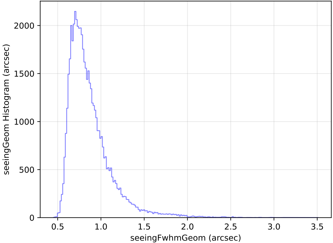
internal_u_expt45_nscale1.1v3.4_10yrs Yr 1 i band: seeingGeom Histogram
